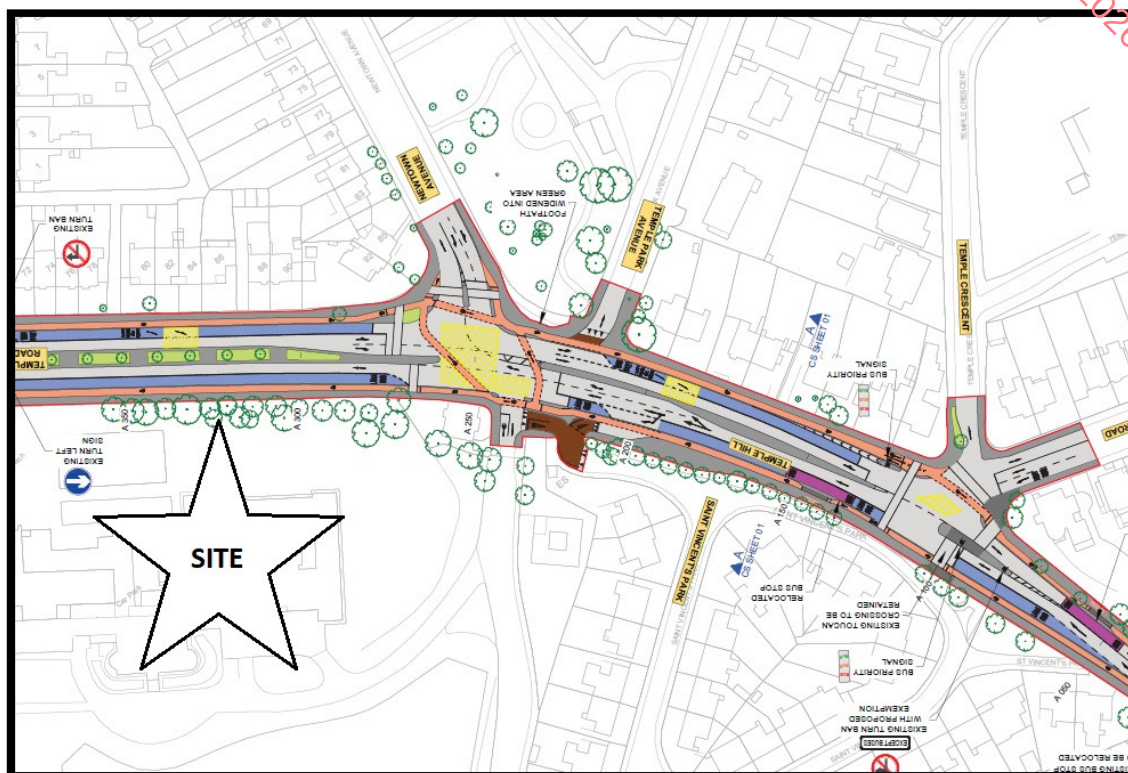
Figure 2.6 – Approved NTA Scheme Design (NTA / ARUP extract)
